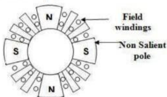
Smooth cylindrical or non salient type rotor
