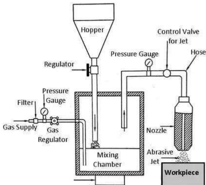
Principle of Abrasive Jet Machining
