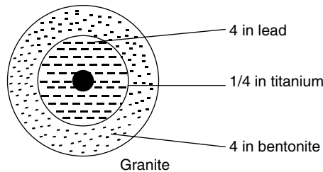
Fig. 16.35 Canister for Vitrified High-Level Waste
