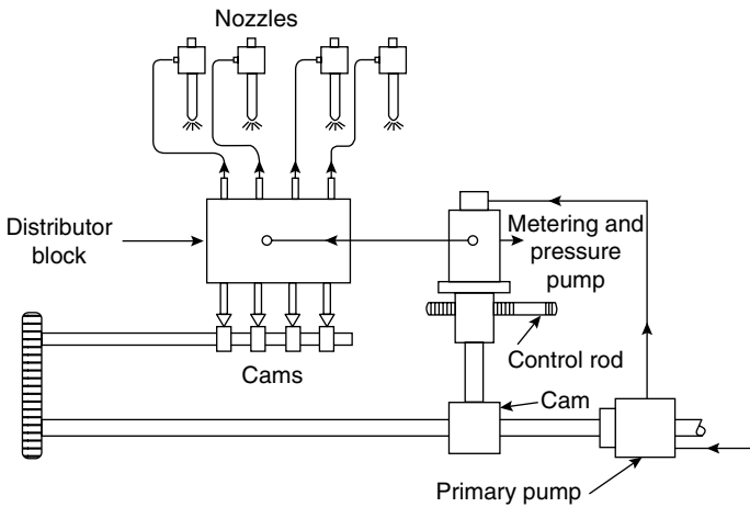
Fig. 13.12 Distributor System
