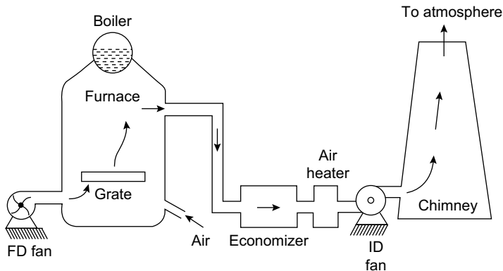
Fig. 7.3 Balanced Draught
